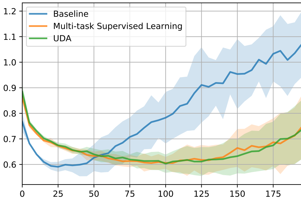
Validation Loss
